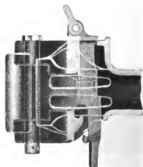
Fig. 3973. R. E. Janney Coupler, Locked.
